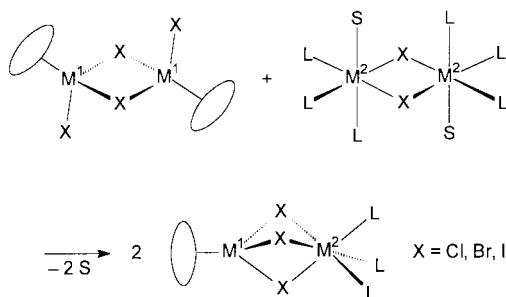
Scheme 1 General method to synthesize heterometallic complexes with three halogeno-bridges: "S" represents a free co-ordination site or a labile ligand, the circle a \pi ligand such as \eta^6 -arene or \eta^5 -cyclopentadiene.
